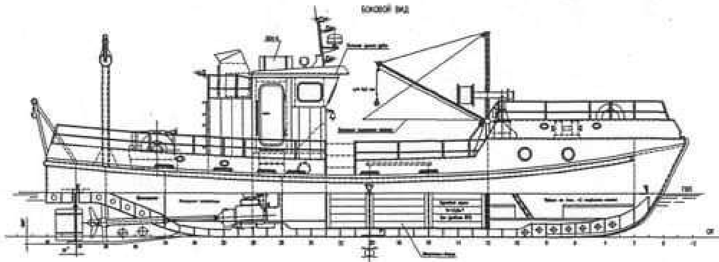
THE DRAWING IS OTHER THAN FROM A PERSPECTIVE POINT OF VIEW AND IS NOT TO BE USED AS SUCH
