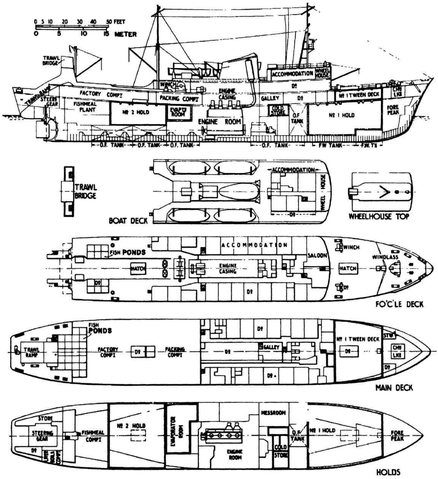
Fig. 604. Arrangement of Fairtry
