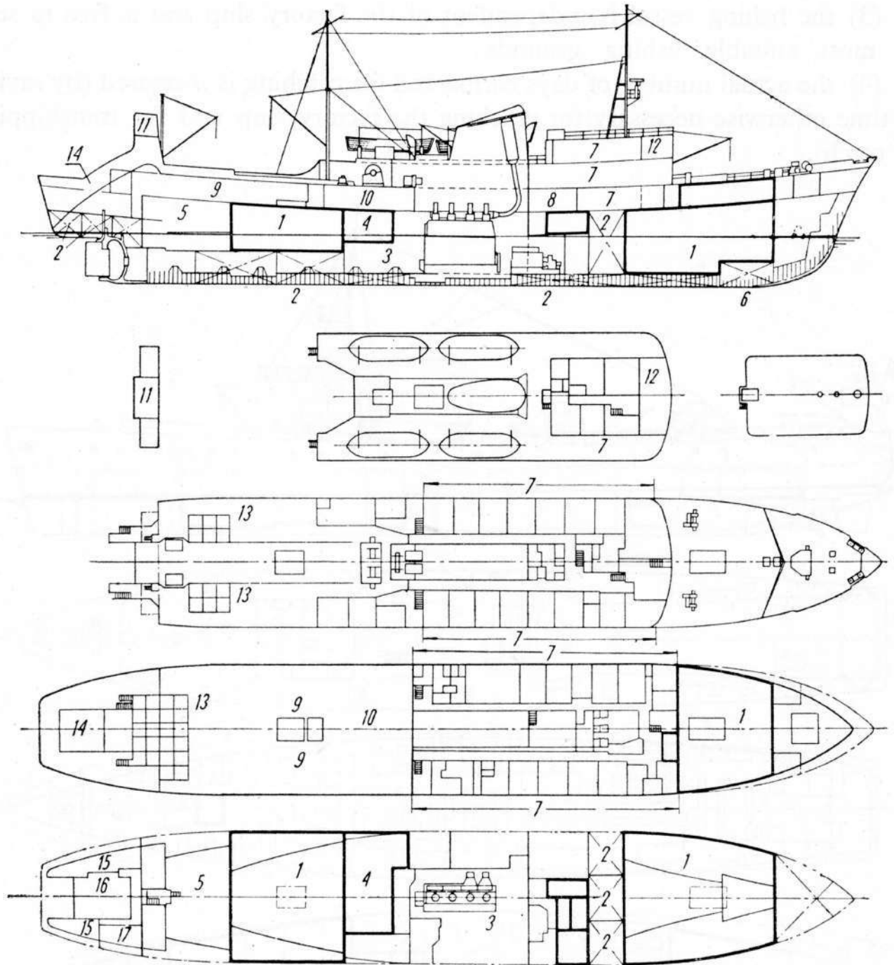
Fig. 34. Fairtry , factory trawler built in Scotland in 1954 at the J. Lewis shipyard in Aberdeen. This is the first ever ship to be built especially for stern fishing and equipped with installations for mechanical filleting and freezing: 1 — hold; 2 — fuel tank; 3 — engine room; 4 — refrigerating plant; 5 — fish meal plant; 6 — fresh-water tank; 7 — crew's quarters; 8 — galley; 9 — processing plant; 10 — packing department; 11 — stern wheelhouse; 12 — wheelhouse; 13 — deck fish-sorting appliances; 14 — stern ramp; 15 — store; 16 — steering gear; 17 — liver oil plant.
